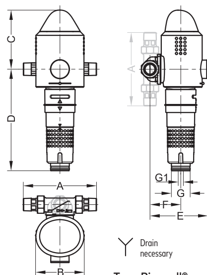
Type Bioquell®- FILT BP ¾" - 1¼"
