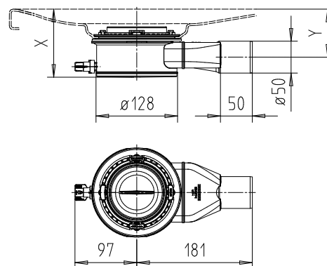
KA 120 HORIZONTAL
