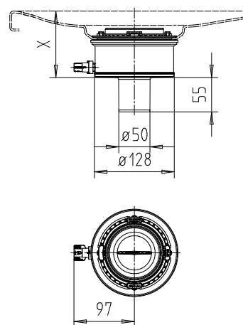
KA 120 VERTICAL
